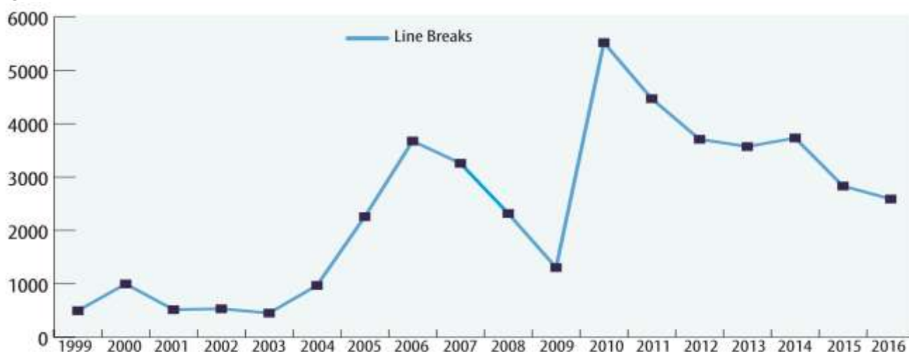
Figure 7.2 Pipeline breaks
